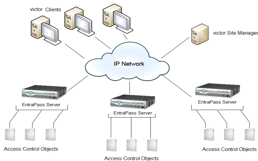
Figure 3-1 System Overview
