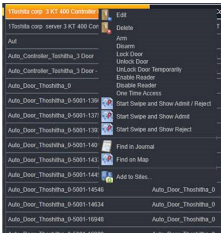
Figure 5-8 Manual actions: Doors
